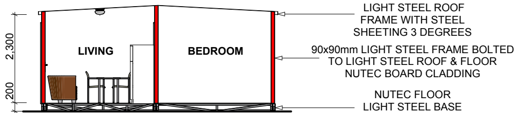
SECTION A
