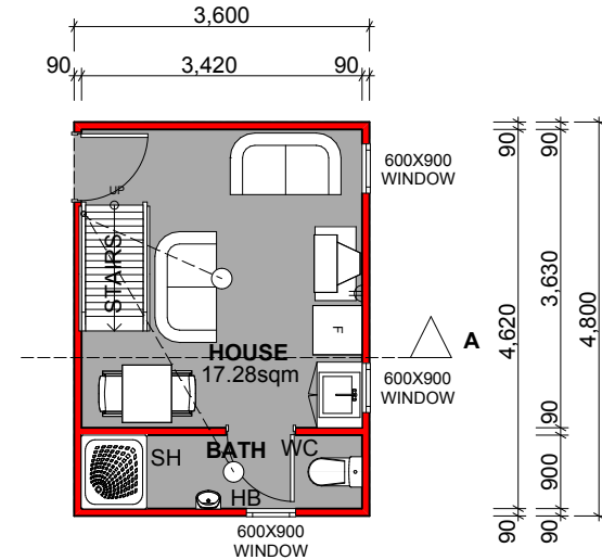
TOTAL 34.56sqm GROUND FLOOR UNIT D
