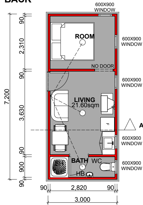
GROUND FLOOR UNIT C
