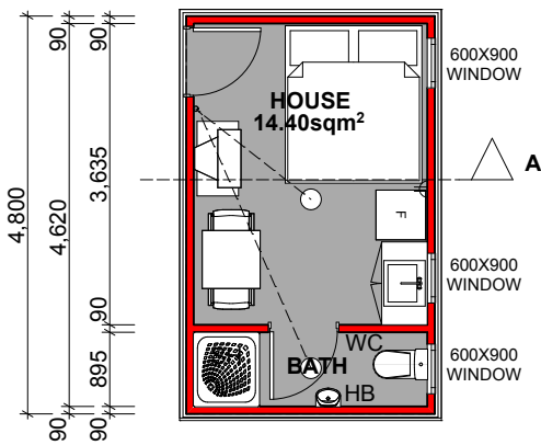
GROUND FLOOR UNIT B
